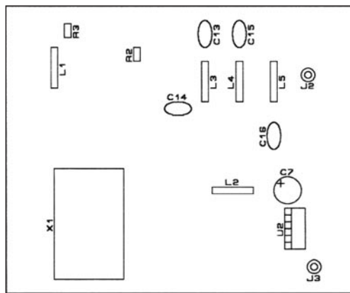
7 - Implantation composants DDS face 2
