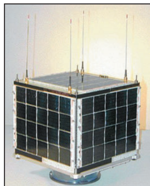
Figure 2: Le satellite OSCAR 51.
