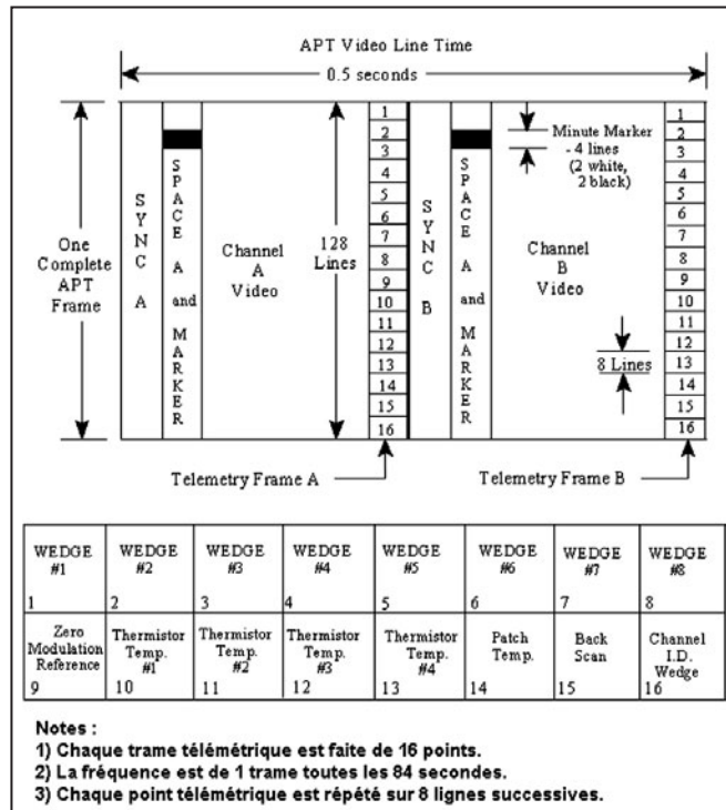
Fig. 3 - APT = Automatic Picture Transmission.
