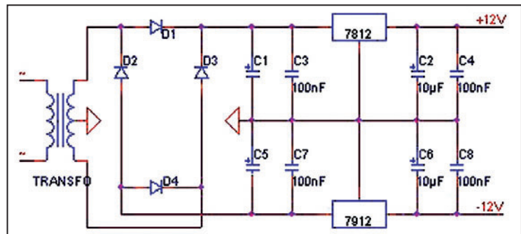
Figure 13: Alimentation 12 V.
