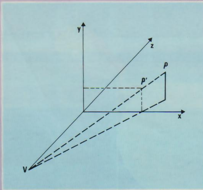
Fig. 5. - Projection perspective.
